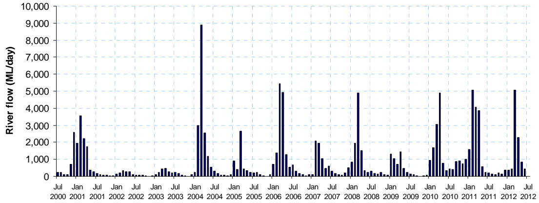
Figure 40. Average daily flow (ML day -1 ) per month from the Annan River. Annan River discharges recorded at Beesbike (DERM station 107003A, 15.68773S, 145.2085 E, Elev:115m) (source The State of Queensland (Department of Environment and Resource Management) 2012, watermonitoring.derm.qld.gov.au ).
