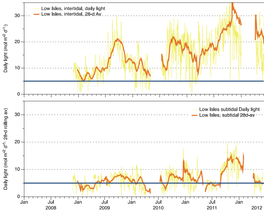
Figure 73. Daily light (28 day rolling average) at inshore intertidal (top) and subtidal (bottom) reef habitats (Low Isles), also showing approximate light threshold required for positive growth in Halodule uninervis dominated communities in the northern GBR ( 5 \text{ mol m}^{-2} \text{ d}^{-1} ) (Collier, et al. 2012b). NB threshold is based on 90 day average.
