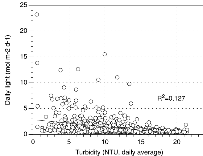
Figure 77. Turbidity (NTU, daily av) and light (daily sum, mol m -2 d -1 ) at inshore subtidal reef habitat (Green Island) since turbidity loggers have been deployed on site (October 2009 onwards)
