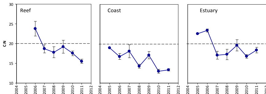
Figure 17. Elemental ratios (atomic) of seagrass leaf tissue C:N for each GBR habitat each year (foundation species pooled). Horizontal dashed line on the C:N ratio panel represents the accepted guideline seagrass “Redfield” ratio of 20:1 (Abal, et al. 1994; Grice, et al. 1996). C:N ratios below this line may indicate reduced light availability and/or N enrichment.
