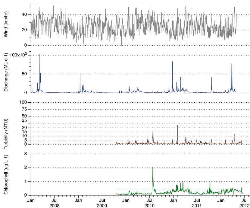
Figure 78. Daily mean chlorophyll concentration (green line, ug L -1 ), turbidity (brown line, NTU) at inshore subtidal reef habitat (Green Island) in the Wet Tropics Region. Additional panels are daily discharge (Russell Mulgrave, ML d -1 x10 5 ) and daily wind speed. Horizontal green and red lines are the GBR Water Quality Guidelines values (Great Barrier Reef Marine Park Authority 2009). Turbidity trigger value (red line) was derived by transforming the suspended solids trigger value (see Schaffelke, et al. 2009).
