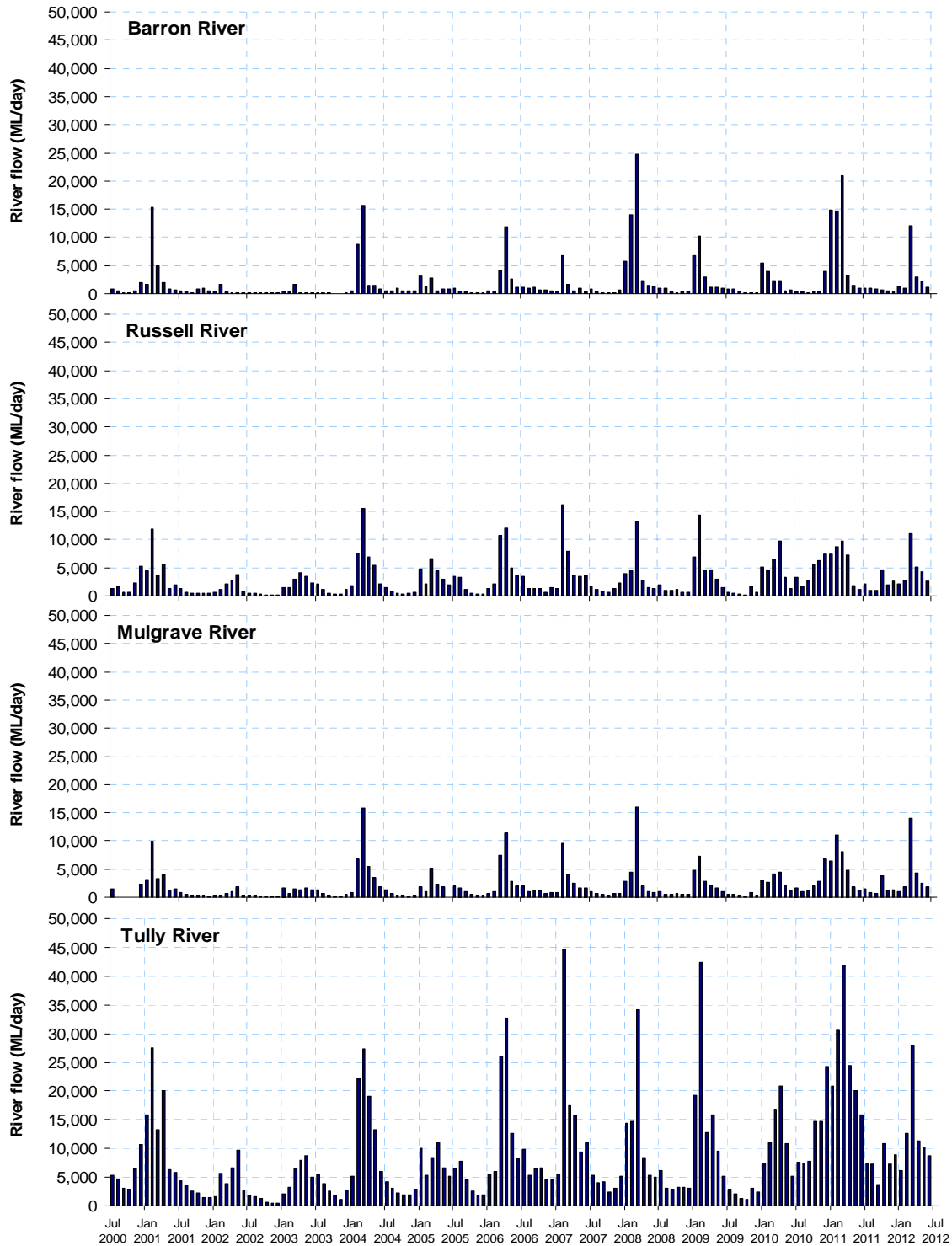
Figure 83. Average daily flow ( ML\ day^{-1} ) per month from the main rivers impacting the seagrass monitoring sites in the Wet Tropics (DERM station 110001D - Barron River at Myola, 16.79983333^{\circ}S\ 145.61211111^{\circ}E , Elev 345m; 111007A - Mulgrave River at Peets Bridge, 17.13336111^{\circ}S\ 145.76455556^{\circ}E , Elev 27.1m; 111101D - Russell River at Bucklands 17.38595^{\circ}S\ 145.96726667^{\circ}E , Elev 10m; 113006A - Tully River at Euramo, 17.99213889^{\circ}S\ 145.94247222^{\circ}E , Elev 8.76m) (source The State of Queensland (DERM) 2012, watermonitoring.derm.qld.gov.au ).
