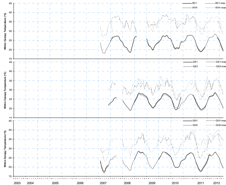
Figure 162. Monthly mean and maximum within seagrass canopy temperature (°C) at inshore intertidal coastal (Shoalwater Bay), reef (Great Keppel Island) and estuary (Gladstone Harbour) habitats within the Fitzroy region.
